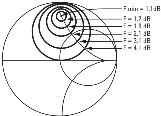
Figure 2-2. Noise circles
